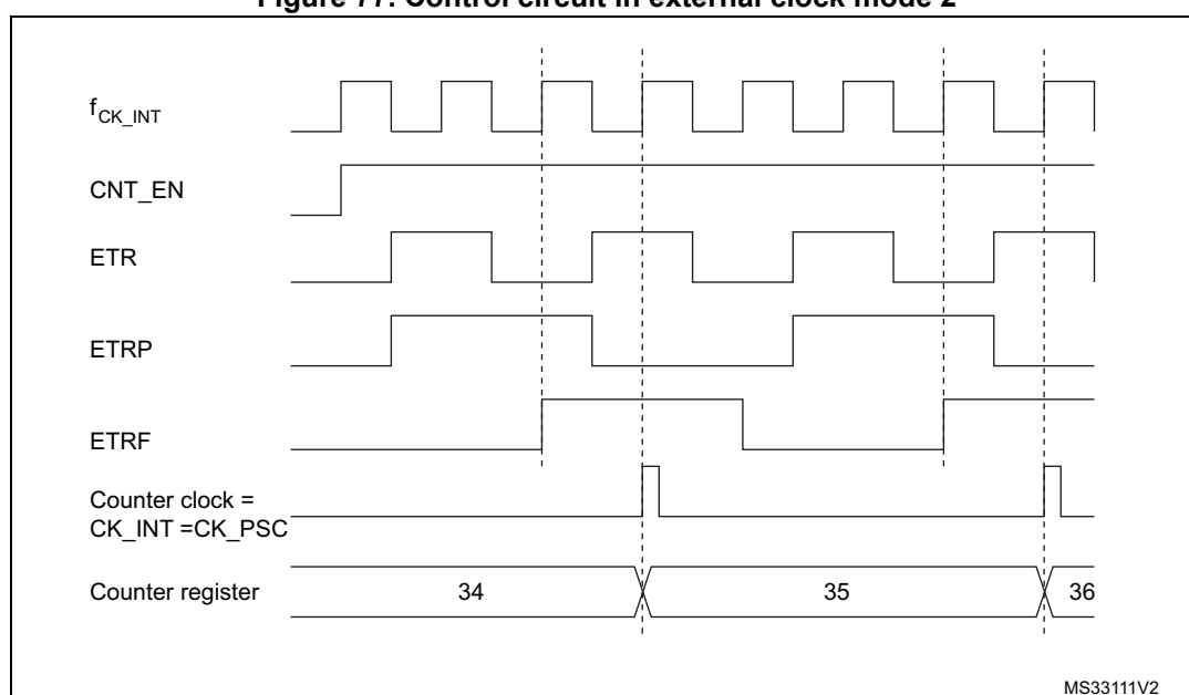
Figure 77. Control circuit in external clock mode 2
