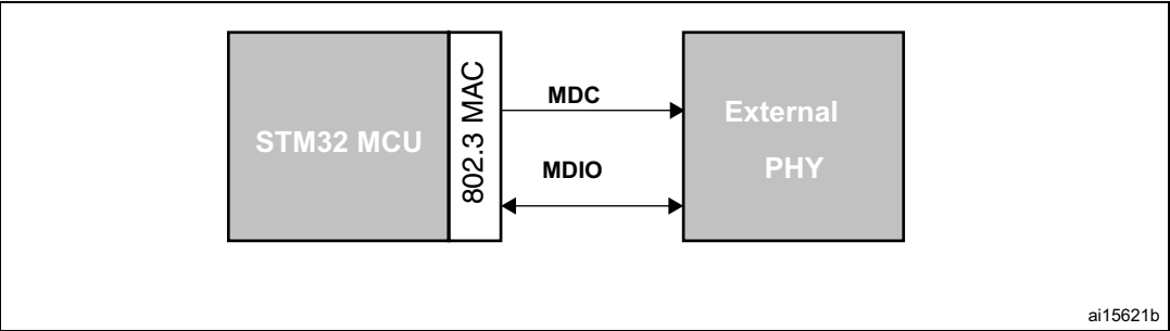
Figure 328. SMI interface signals
