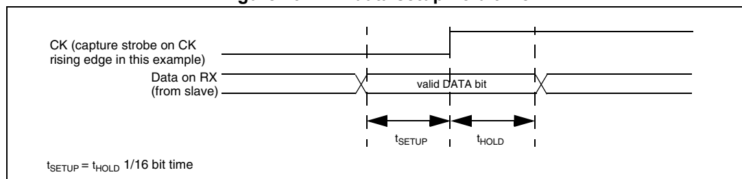
Figure 292. RX data setup/hold time
