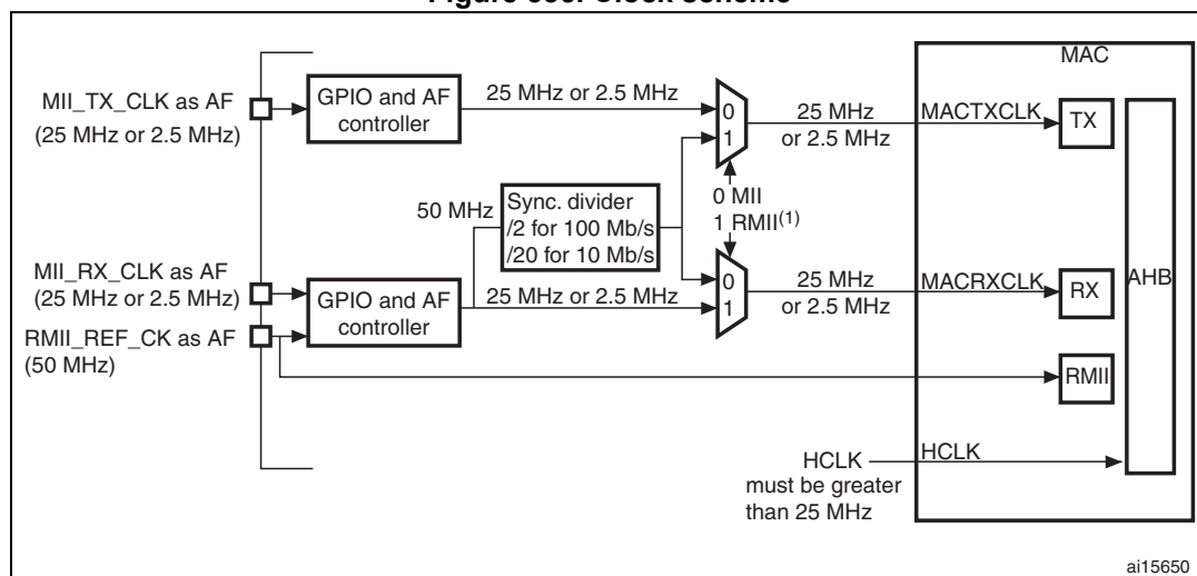
Figure 335. Clock scheme
