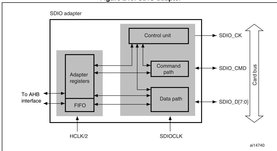
Figure 213. SDIO adapter
