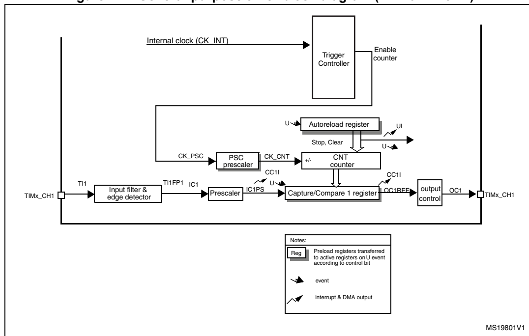
Figure 147. General-purpose timer block diagram (TIM10/11/13/14)
