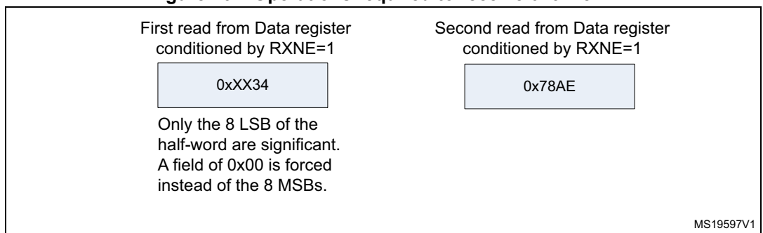
Figure 262. Operations required to receive 0x3478AE
