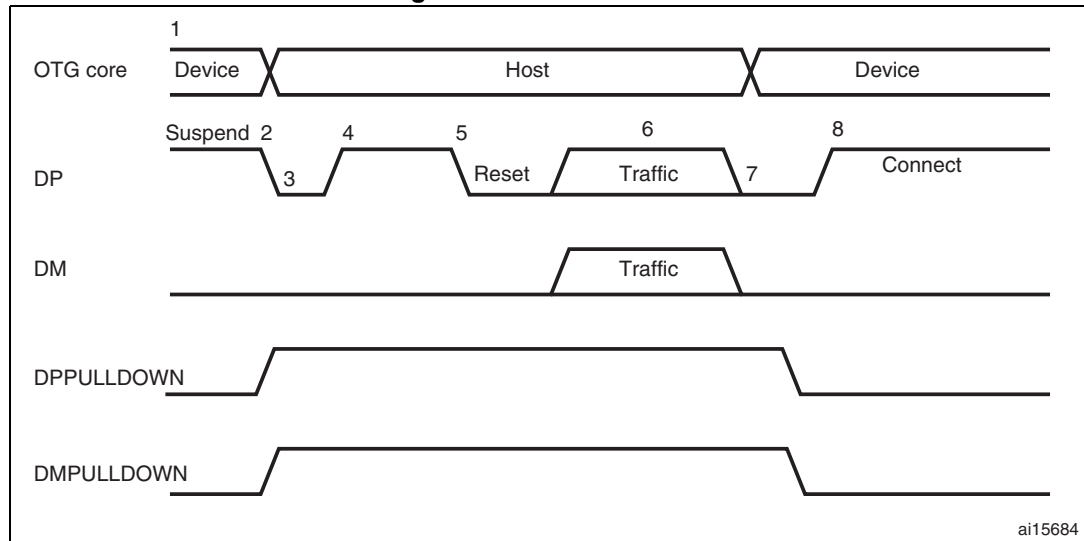
Figure 326. B-device HNP
