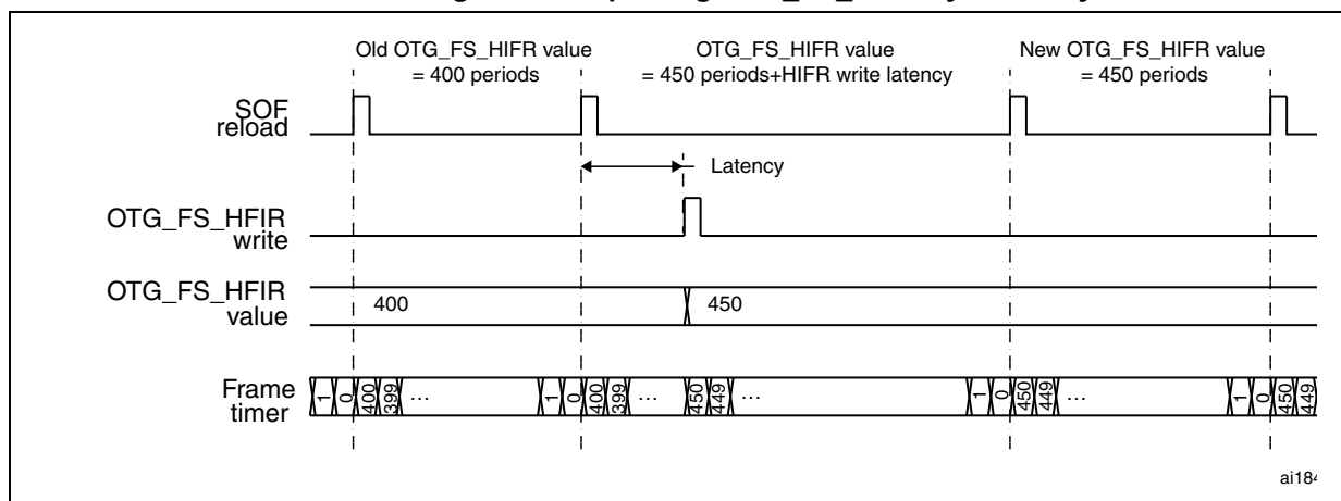
Figure 308. Updating OTG_FS_HFIR dynamically
